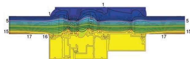
➤ INFINEO THERMIQUE NOEUD CENTRAL
