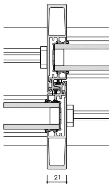
› INFINEO MONTANT CENTRAL
