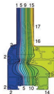
➤ INFINEO THERMIQUE NOEUD VERTICAL
