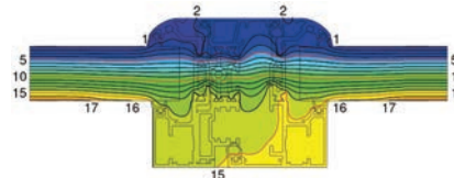
➤ INFINEO THERMIQUE NOEUD CENTRAL
